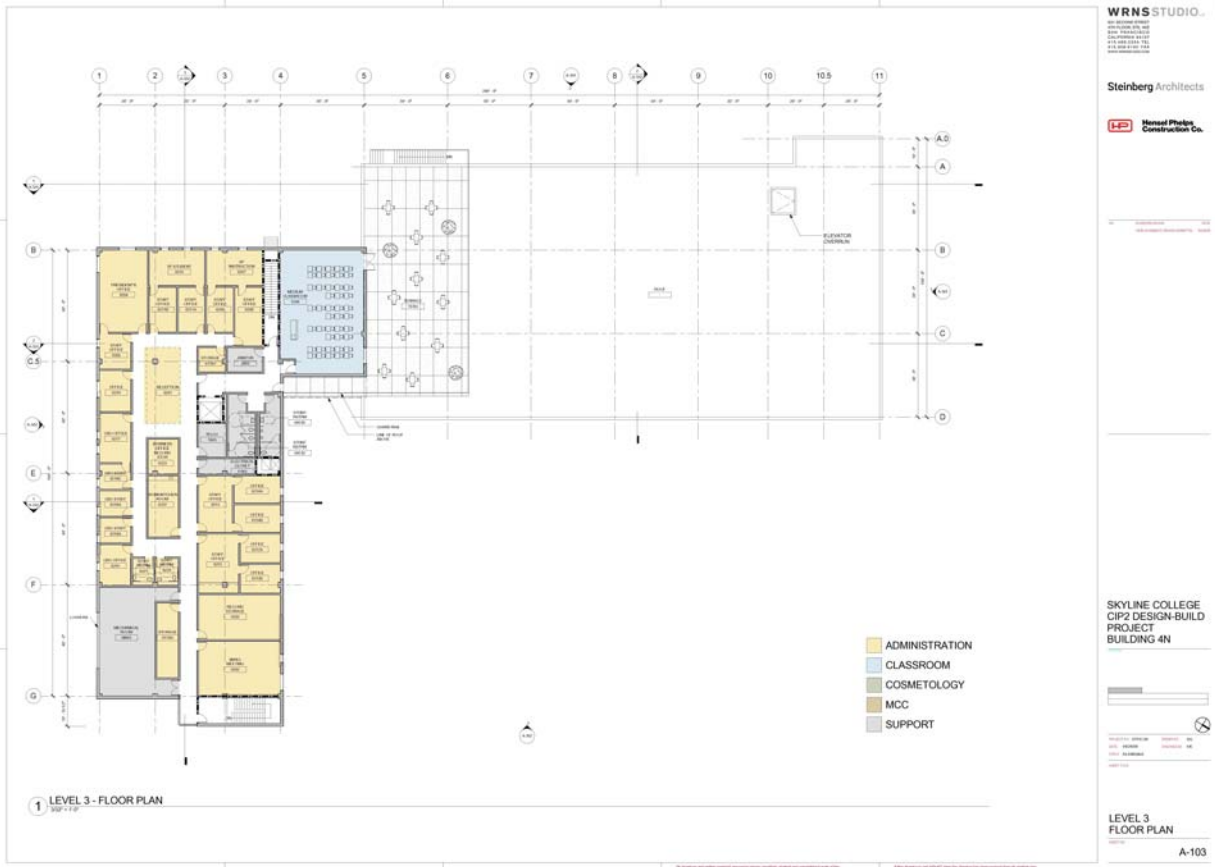
Building 4N, Level Three (top of plan is west)
