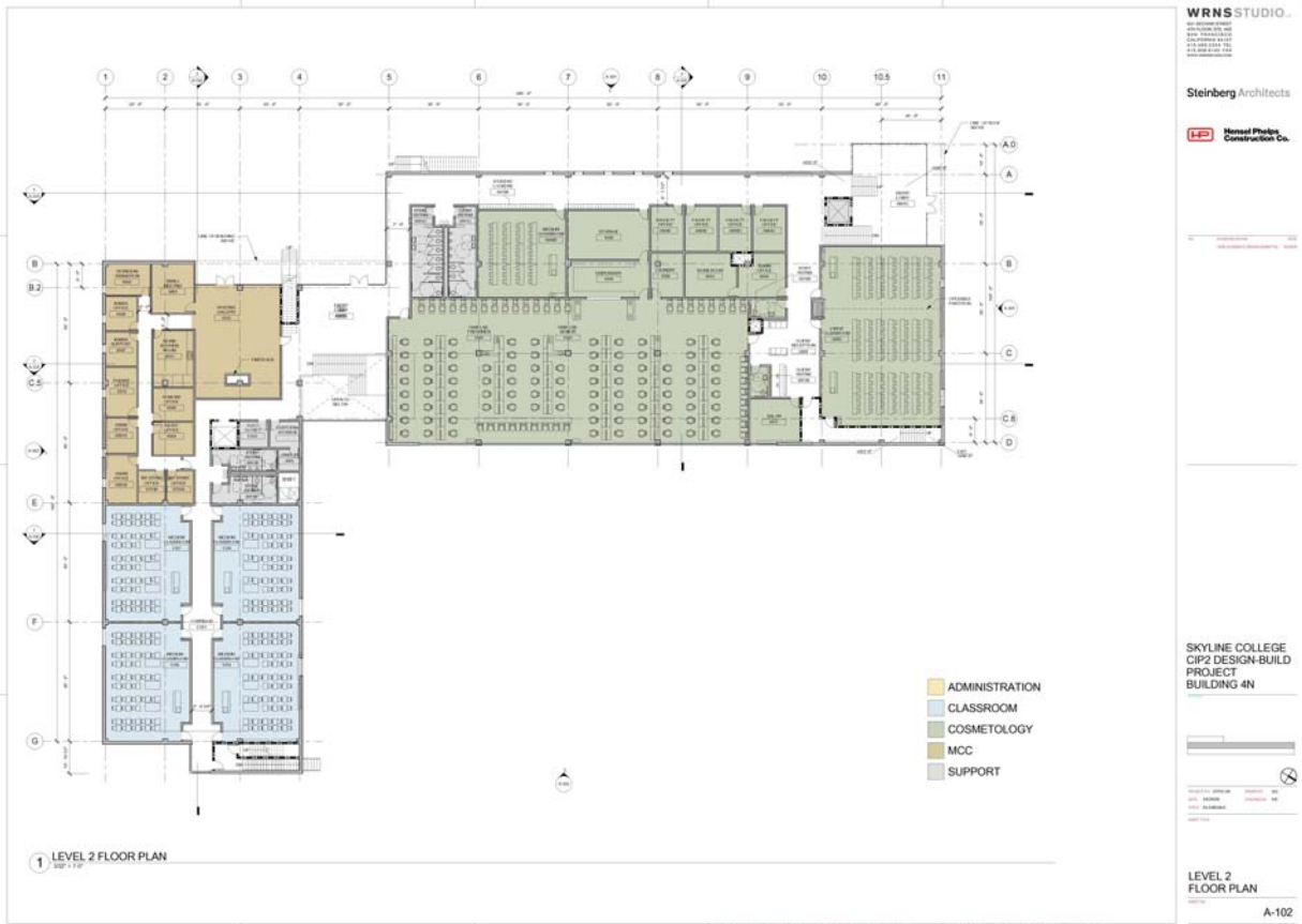
Building 4N, Level Two (top of plan is west)
